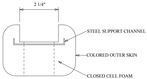
SECTION VIEW A
