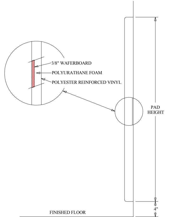
WALL PAD WITHOUT NAILING FLANGE
