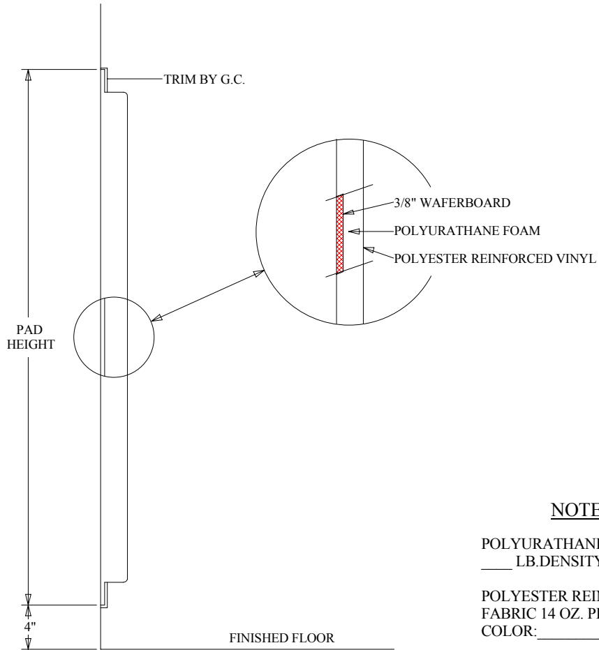
WALL PAD WITH NAILING FLANGE
